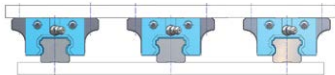
Three-rail arrangement (3)
