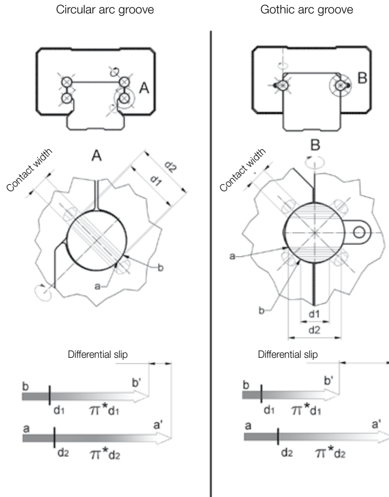
Figure 1.3 Groove geometry
