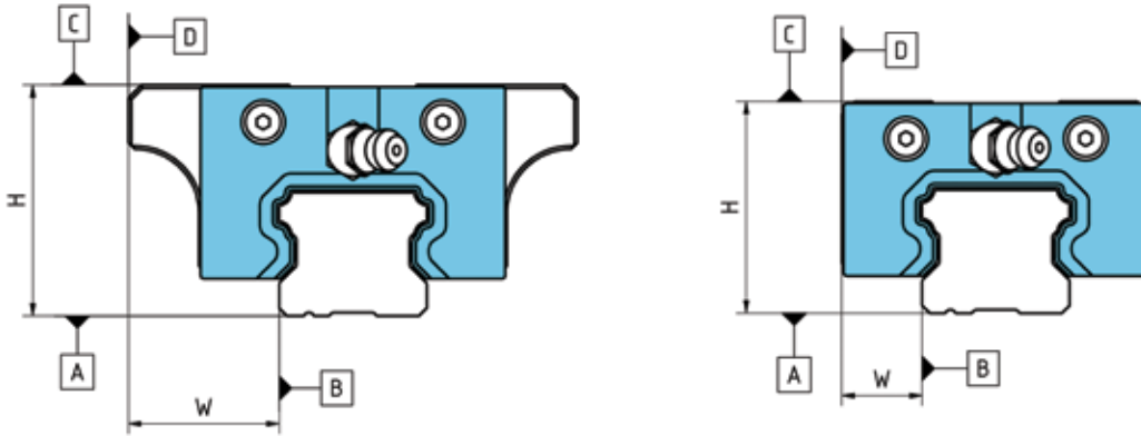
Figure 2.20 Precision classes
