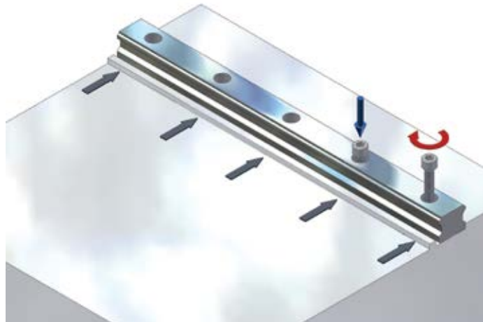
Figure 3.11 Pre-installing
