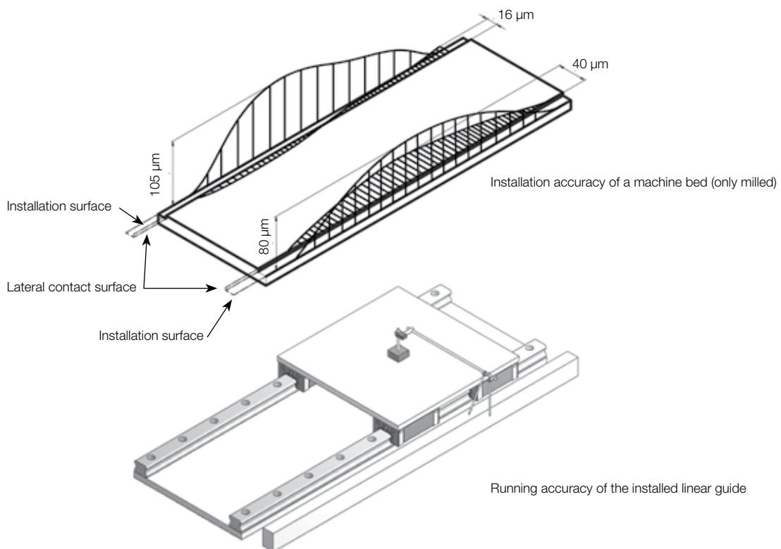
Figure 2.23 Error compensation
