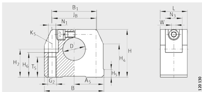
GWH..-B
