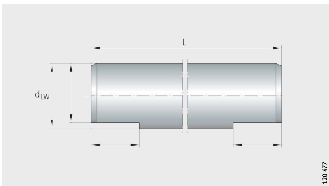
Figure 13 Flattened area
