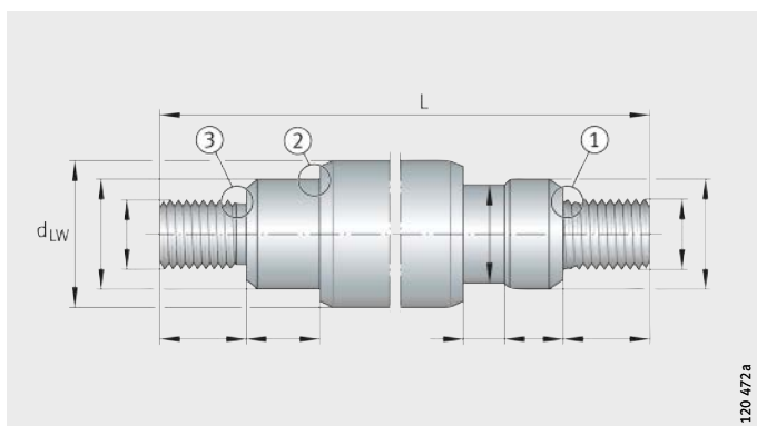
Figure 9 Journal and threaded journal
