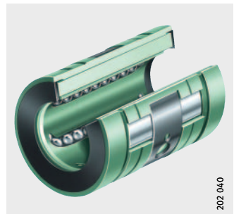
KNO...-B, KNO...-B-PP
