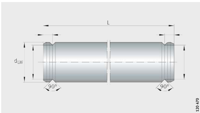
Figure 7 90° undercut
