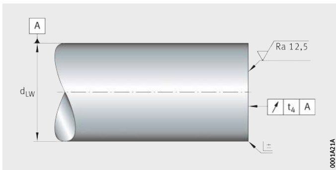
Figure 16 Parting cut
