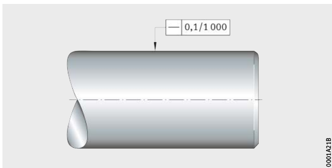
Figure 17 Straightness
