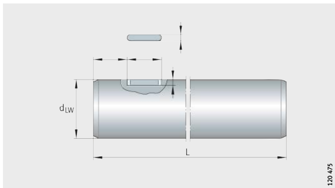
Figure 11 Keyway
