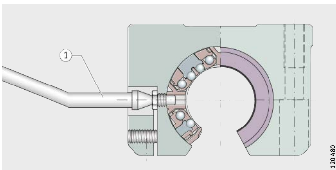
① Nozzle tube
