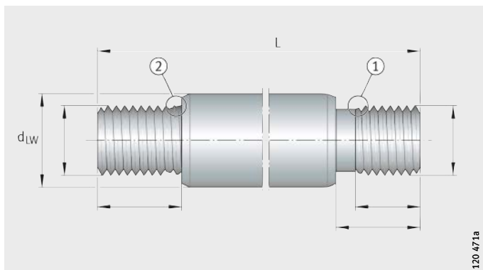
Figure 8 Threaded journal
