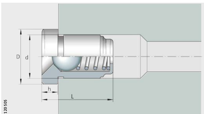
Figure 6 Lubrication nipple for compact range KH, machined range KB, plain bearing range PAB
