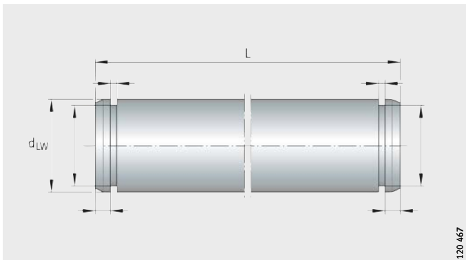
Figure 4 Undercut for retaining ring
