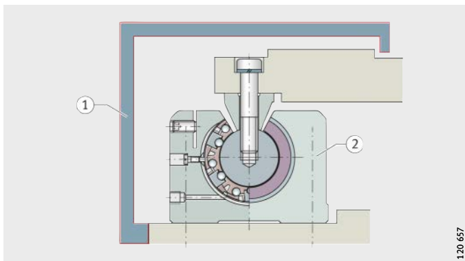
Figure 7 Suspended shaft guidance system with drop guard
