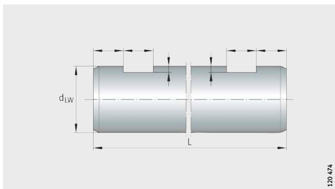
Figure 10 Slot
