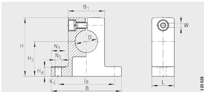
GW, GWA..-B
