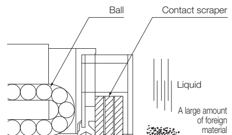
Structural Drawing
