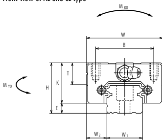
Front view of AL and CL type
