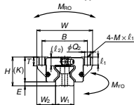
Front view of EM and GM types
