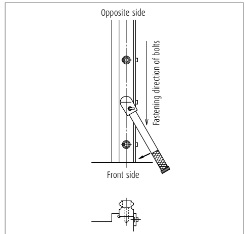
Fig. 14 Rail installation
