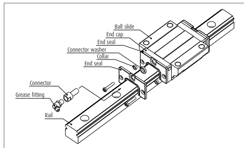
Fig. 12 Double seal
