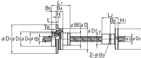
Ball screw unit (Models NS 0812A and 1015A) Ball spline (Models NS 0812A and 1015A)
