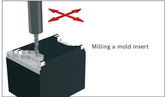
Hard milling
